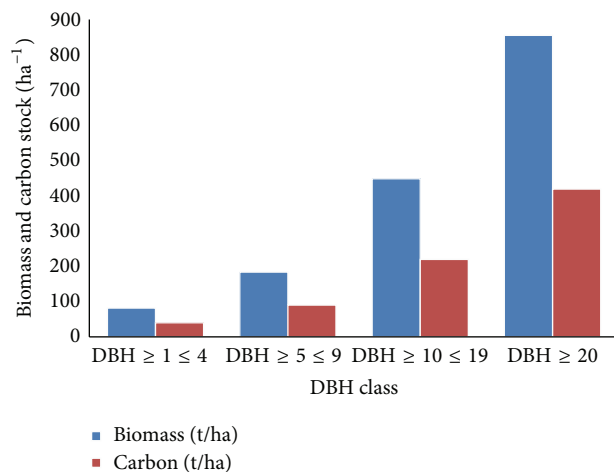
FIGURE 2: Above ground biomass and carbon stock distribution in Mnesia forests, Kolo Hills, Kondo.
