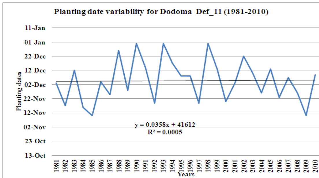
Figure 7: Planting date variability for Dodoma in Def_11 from 1981-2010
