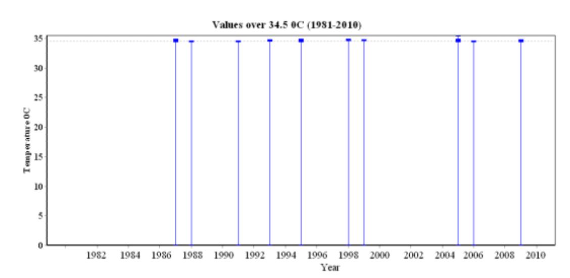
Figure 21: Temperature values exceeding 34.5^{\circ}\text{C} by years in the study site
