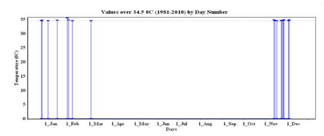
Figure 20: Temperature values exceeding 34.5^{\circ}\text{C} by day number in the study site
